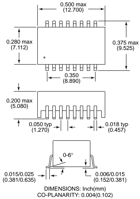
SMD Package
