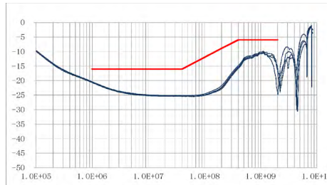
Return Loss
