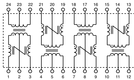
Circuit B
