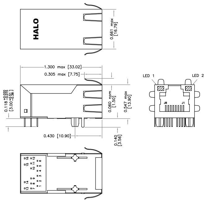
Dimensions are in inch [mm]
