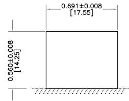
RECOMMENDED PANEL CUT
